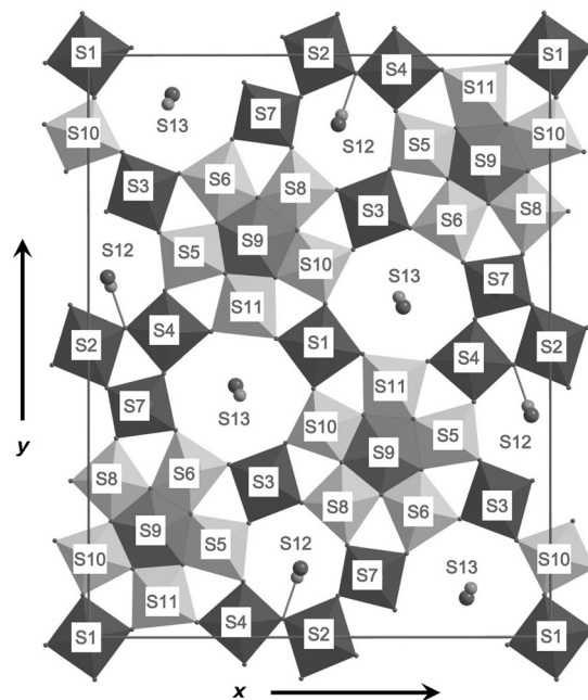
Figure 1. Structure of the M1 phase of MoVTeNbO 4 (orthorhombic) as viewed along the (001) basal plane. The various sites for Mo, V, and Nb atoms are shown as oxygen polyhedra: pentagonal (S9) and octahedral ring sites (light gray), and octahedral link sites (dark gray). Light/dark balls represent the Te/O atoms in the channels.
